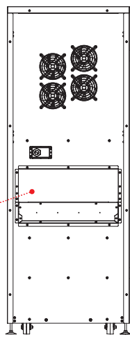
S3U and S3U SW 40-60 kVA (rear)
