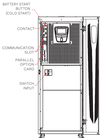
S3U and S3U SW 40-60 kVA (front)
