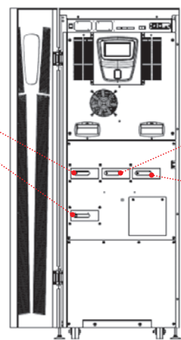
Model S3U 40-60 kVA (front)
